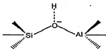
Figure-1: Description of the Chemical Structure of Zeolite
