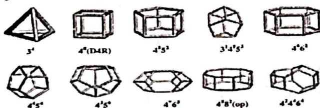
FIGURE 3: Some of the cage building units in zeolites.
